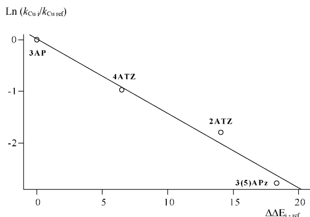
Figure 4. Linear correlation between rate constant for the \text{Cu}^{2+} -catalysed enolization reaction and thermodynamic stability of the substrate-metal ion complexes of 3AP , 2ATZ , 4ATZ and 3(5)APz , with reference to 3AP
