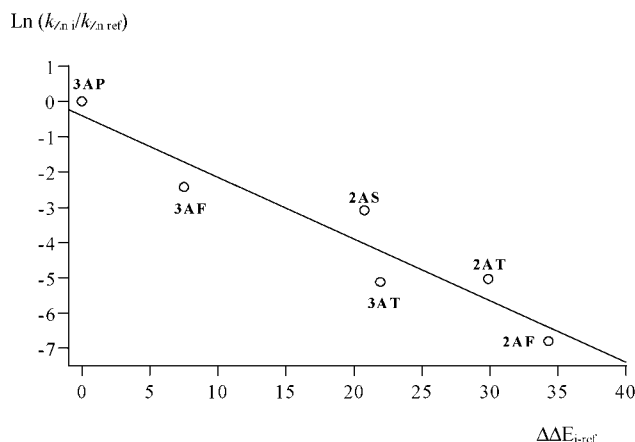
Figure 3. Linear correlation between rate constants for the \text{Zn}^{2+} -catalysed enolization reaction and thermodynamic stability of the substrate–metal ion complexes with reference to 3AP
