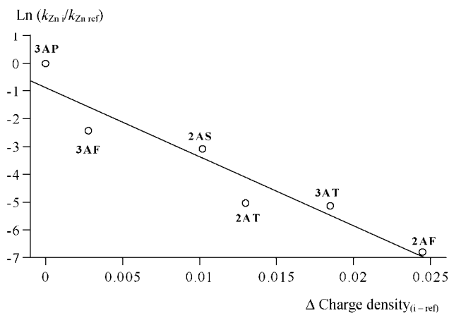
Figure 1. Linear correlation between rate constants for the Zn^{2+} -catalysed enolization reaction and differences in charge densities on the carbonyl oxygen atom, with reference to 3AP , for some acetylheterocycles with one ring heteroatom
