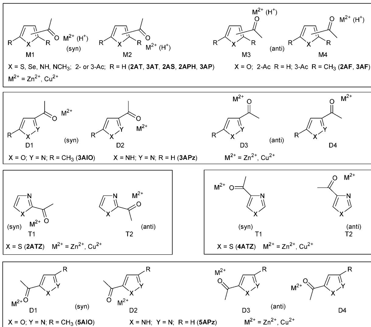
Figure 5. Structures and conformations (syn/anti) of some acetylheterocycles and their adducts with metal ( M^{2+} ) or proton ( H^+ ) ions considered for DFT calculations
