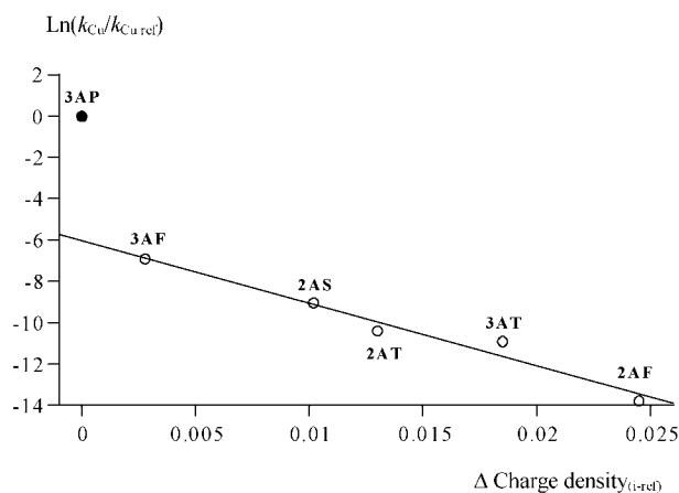
Figure 2. Linear correlation between rate constants for the Cu^{2+} -catalysed enolization reaction and differences in charge densities on the carbonyl oxygen atom, with reference to 3AP , for some acetylheterocycles with one ring heteroatom. Open circles (○) refer to compounds used for drawing the line. 3AP (●) has been excluded from the correlation
